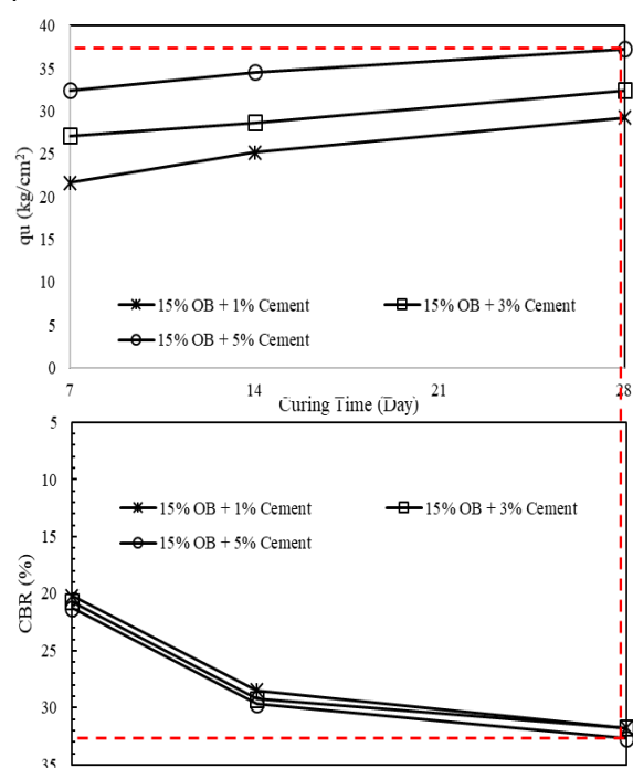
Fig. 2. Recapitulation Relation Of CBR and UCS value of the stabilized soil
